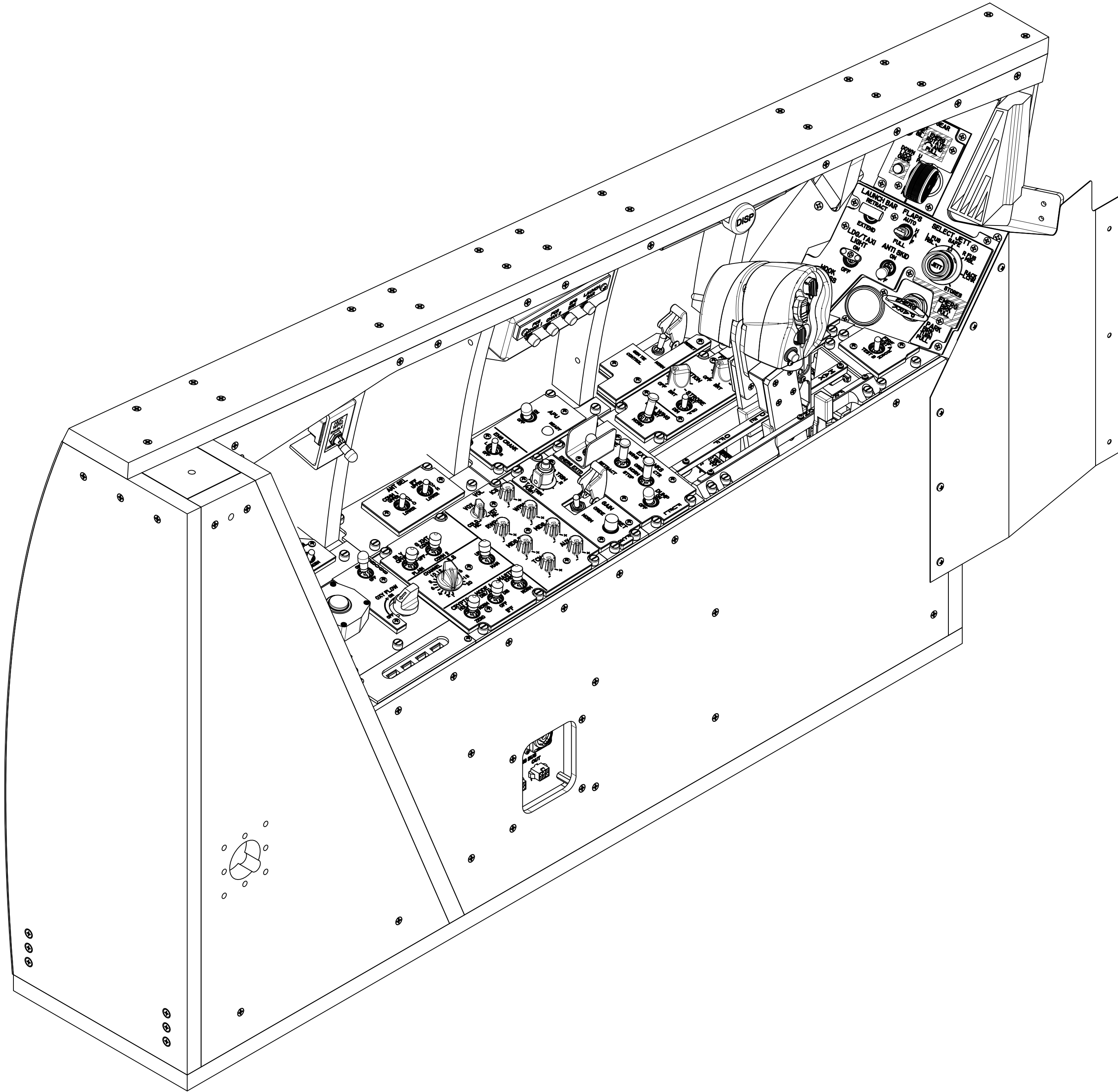
-1 ASSY
